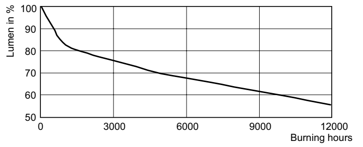
CDM-Tm Elite 20W Lumen Maintenance /830 PGJ5
