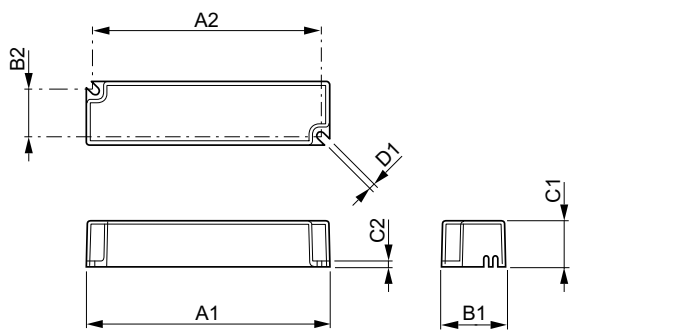
Xtanium 20W/0.7A 277V INTELLIVOLT ROHS
