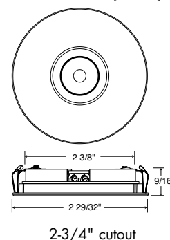
Recessed Mount (USTLR1)
