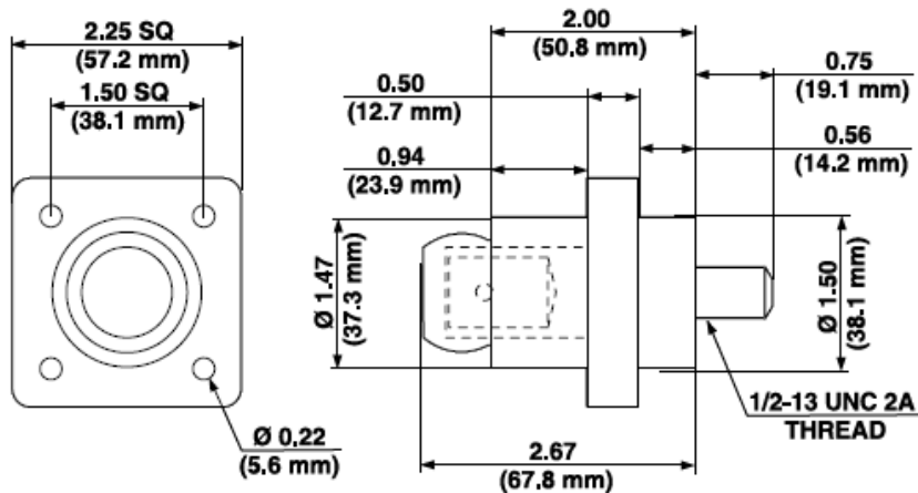
Female Double Set Screw Panel Receptacle
