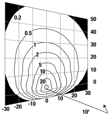
MINILITER V MHS-Y150P8 10' GRIDS WITH 10' SET BACK
