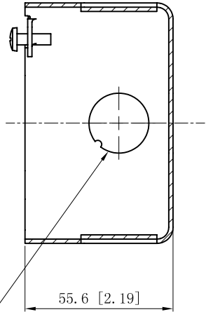
2 1/2" KNOCKOUTS \phi=22.5 [ \phi=0.89 ] CUTAWAY VIEW A-A
