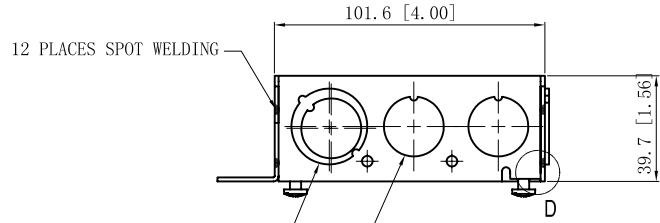
WELDING STYLE DETAIL VIEW D
