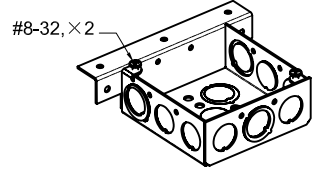
WELDING STYLE DETAIL VIEW D
