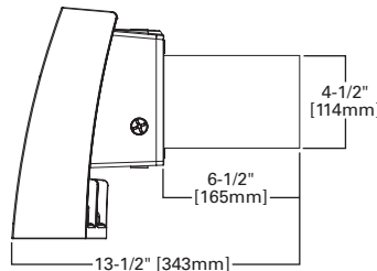
ARM MOUNT
