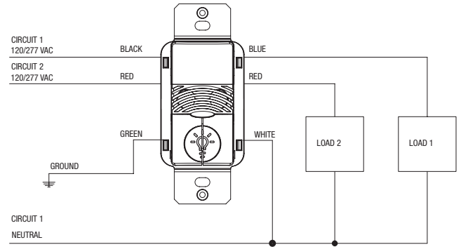
120/277 VAC dual level dual circuit wiring diagram
