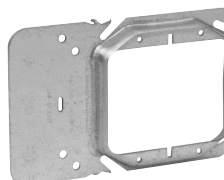
Two Gang
